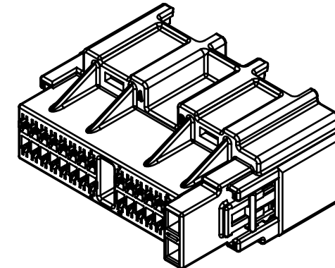
REAR ISOMETRIC VIEW (1/1)
