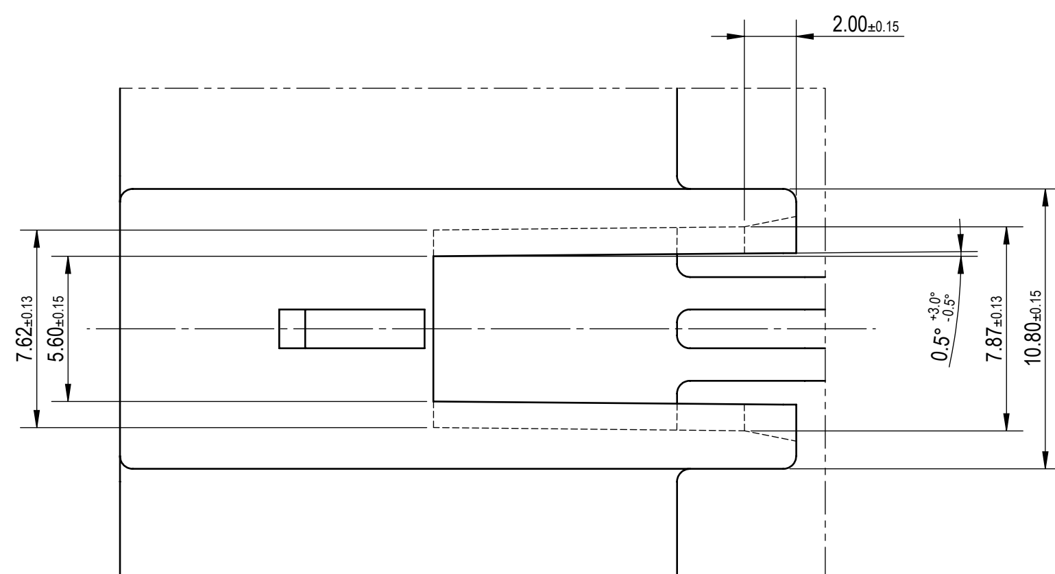
SECTION B-B
