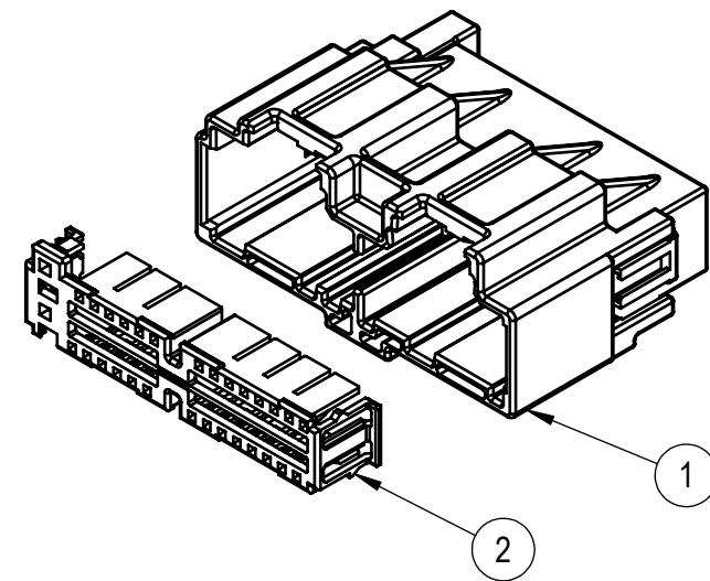
EXPLODED VIEW (1/1)
