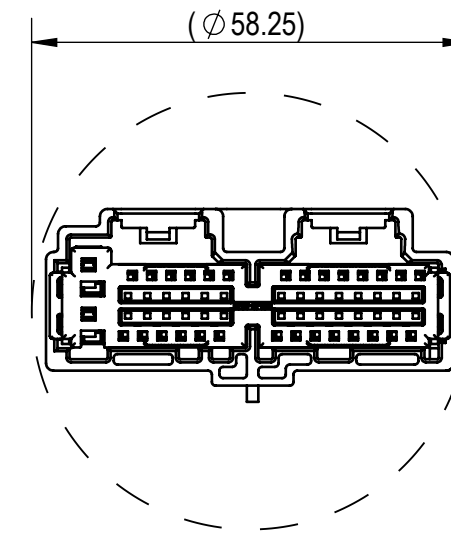
RECOMMENDED PASS-THROUGH HOLE DIMENSION (1mm CLEARANCE ALL AROUND) (1/1)
