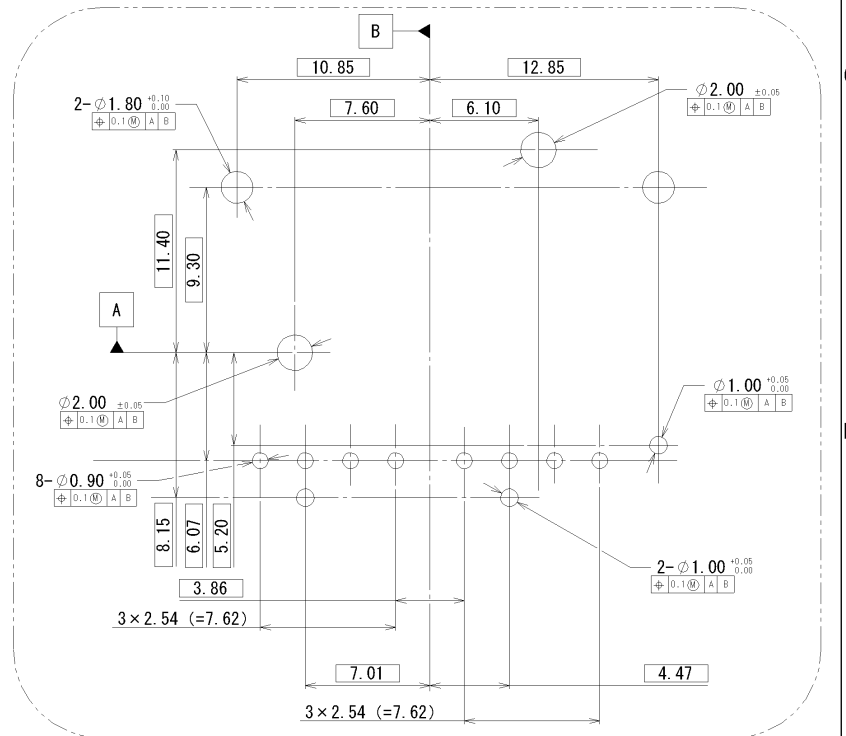
SOLDERING FACE (BOTTOM VIEW) (5/1)
