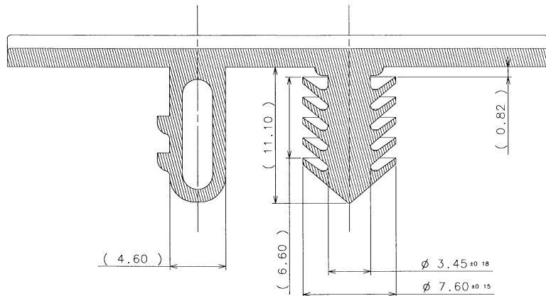
SECTION A-A (5/1)
